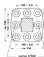
hole pattern 57244
