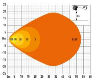
159280 | Lazer Utility 25 LED arbetslampa
