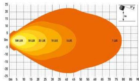
159283 | Lazer Utility 80 LED arbetslampa 159284 | Lazer Utility 80 LED arbetslampa ADR-godkänd
