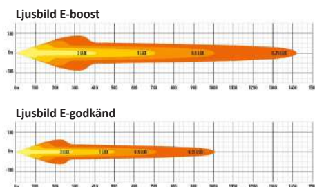
159306 | Lazer Carbon-6 Spot LED extraljusramp 12" (308 mm) 159308 | Lazer Carbon-6 Spot 3D LED extraljusramp 12" (308 mm)
