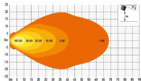
159281 | Lazer Utility 45 LED arbetslampa 159282 | Lazer Utility 45 LED arbetslampa ADR-godkänd
